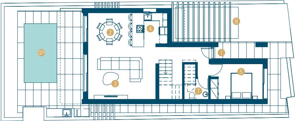
GROUND FLOOR
